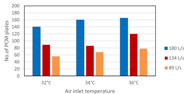
Fig. 12 Number of PCM plates for different air flow rates and outdoor air temperatures.
