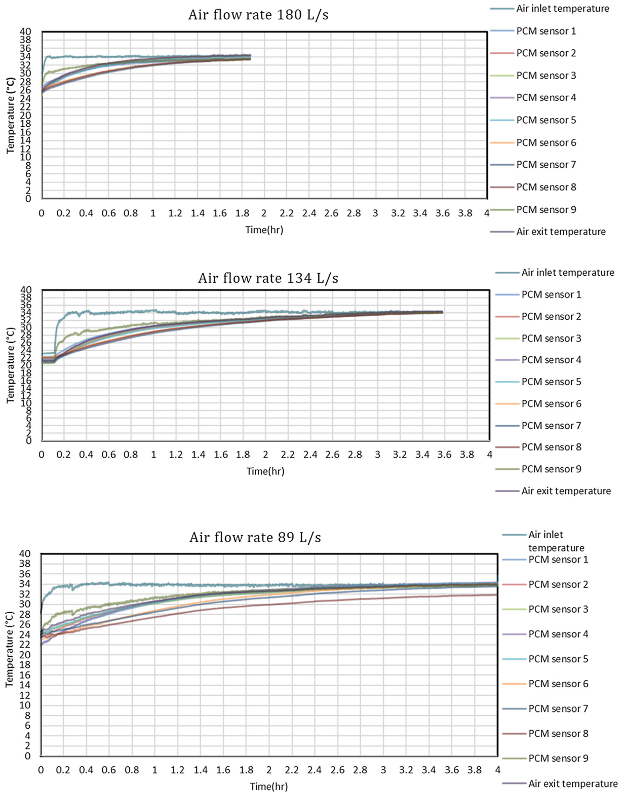
Fig. 6 Temperature distribution at 34 °C air inlet temperature and different air flow rates.
