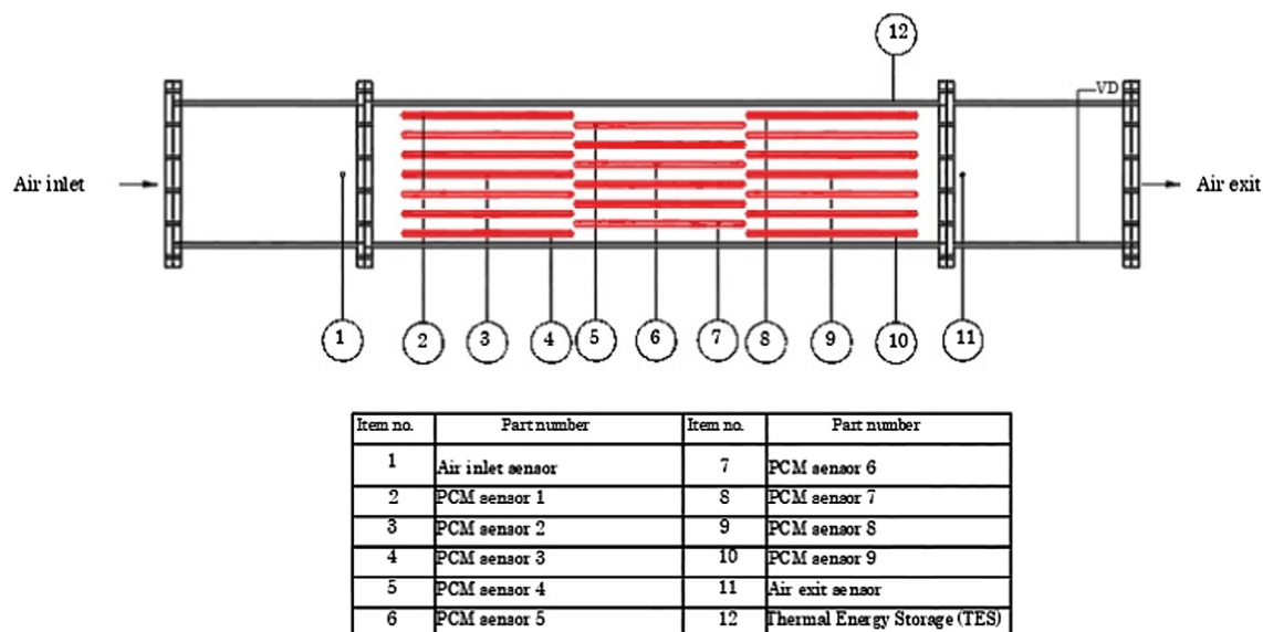
Fig. 3 Thermocouple distribution and the array of the PCM panels in the test section.
