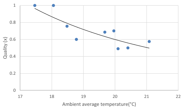
Fig. 9 Assessment of complete solidification of the PCM during night charging.
