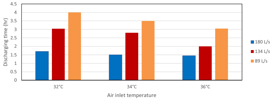
Fig. 11 Effect of air flow rate and air inlet temperatures on the discharge time.
