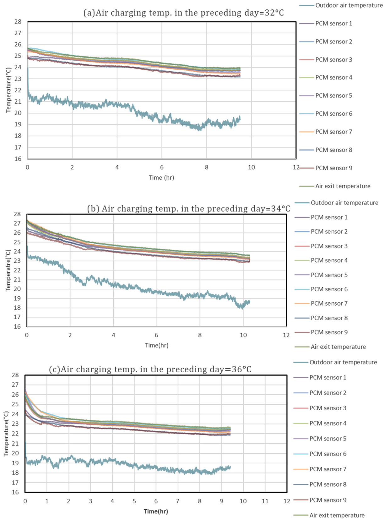
Fig. 8 Charging processes of PCM at 180 L/s and different preceding charging temperatures.
