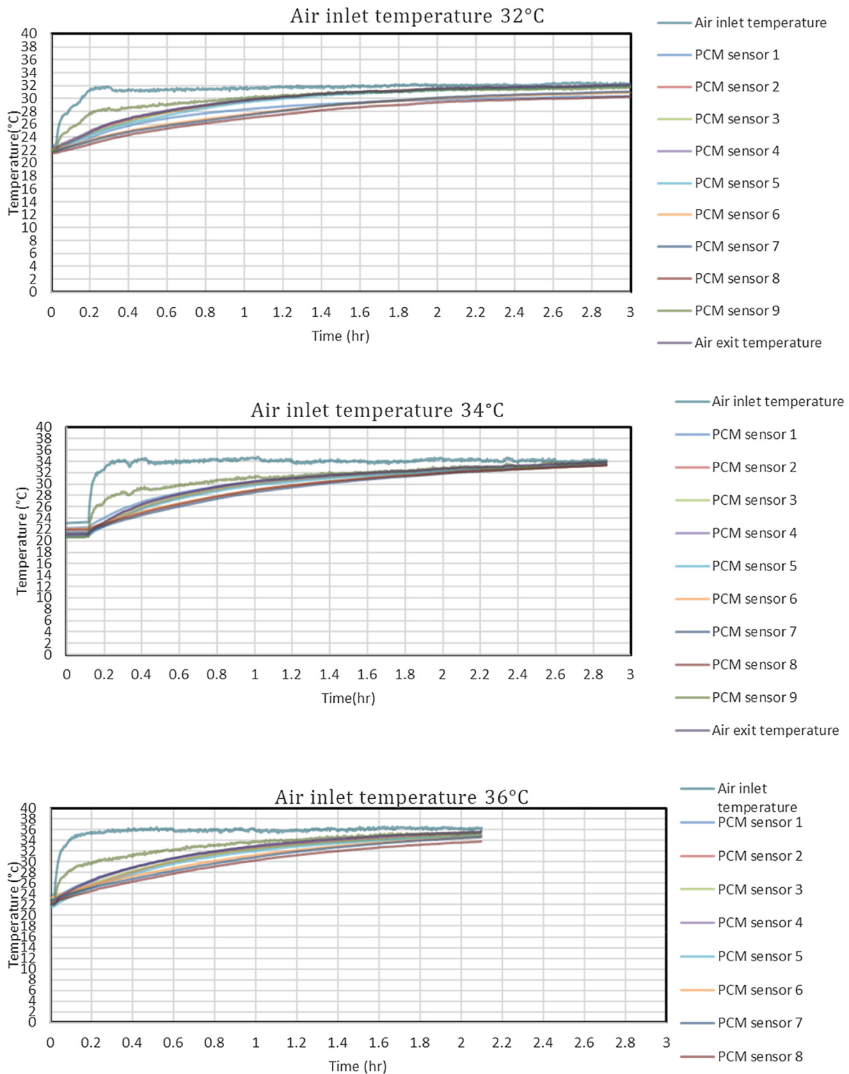
Fig. 7 Temperature distribution at 134 L/s air flow rate and different air inlet temperatures.
